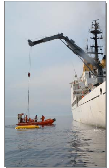
Top: The Alliance underway. Bottom: Retrieving an autonomous underwater vehicle.
